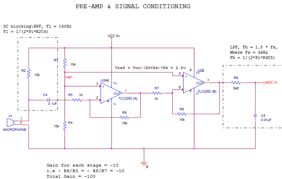
Fig. 2. Amplifier and Signal Conditioning Circuit Diagram
