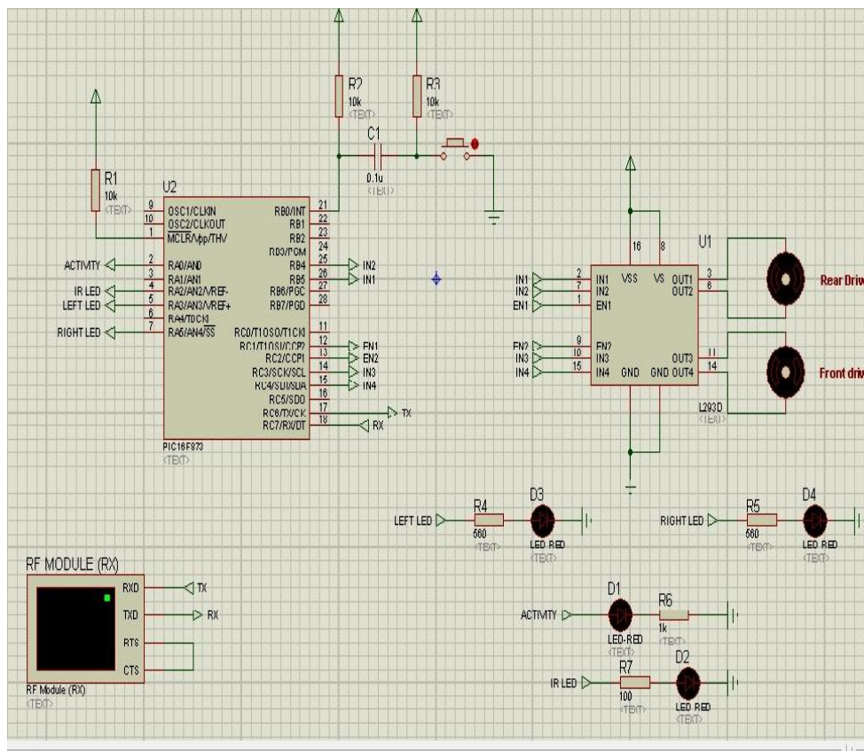
Fig.5. The Trolley Proteus model
