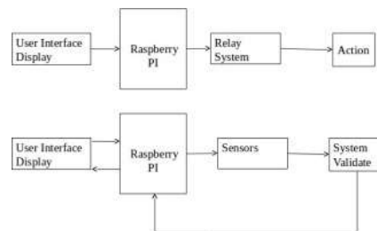
Fig. 5. Block Diagram
