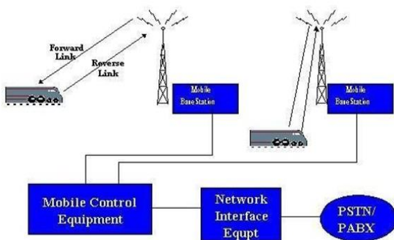
Figure 1: Basic Mobile Telephone Service Network
