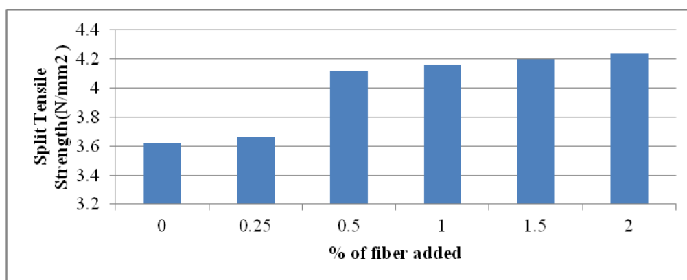
Figure 3: Split Tensile Strength variation
