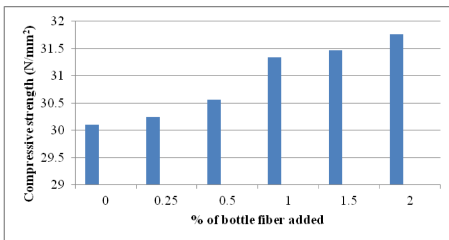
Figure 2: Compressive Strength variation (28 days)
