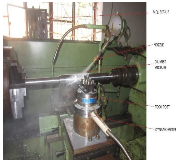
Fig.2: Experimental setup for MQL
