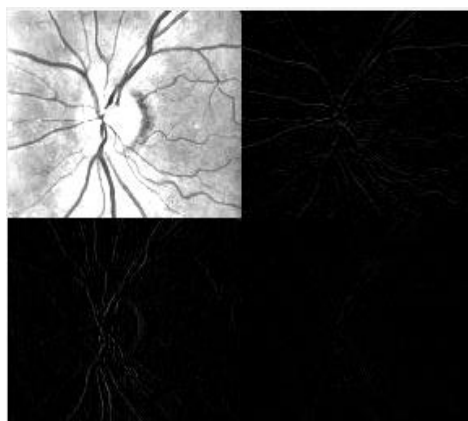
Fig 9: DWT
