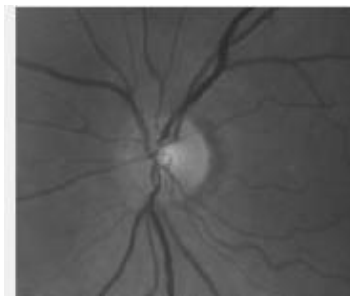
Fig. 5. Wiener Filter
