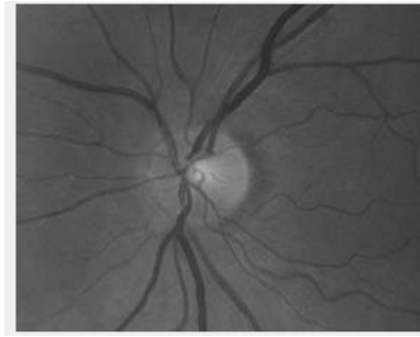
Fig. 4. Gray Image
