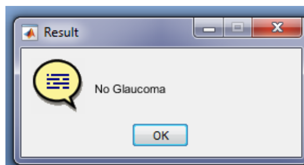
Fig 12 output
