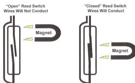
Figure (2) Operation of Reed Switch
