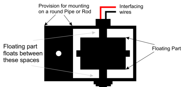
Figure (1) Internal Structure of Reed Switch
