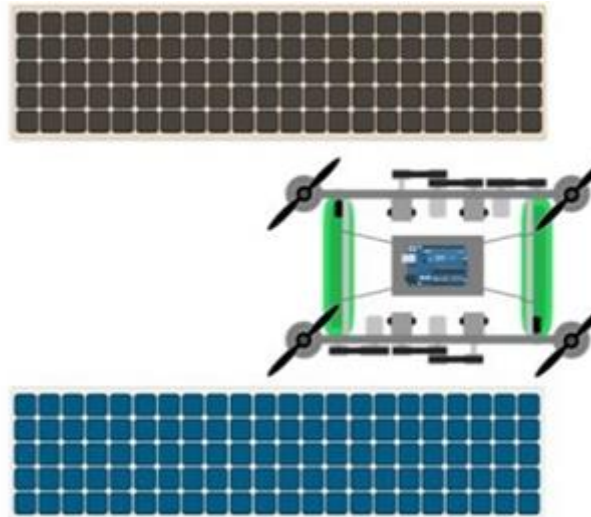
Fig. 10 Autonomous flying solar panel cleaning system.
