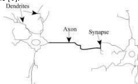
Fig 1: Brain neuron [2]
