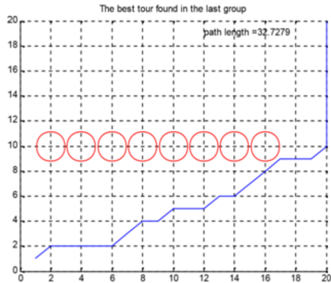
Fig- 7 Optimal Path found with CNN-MH for Experiment3
