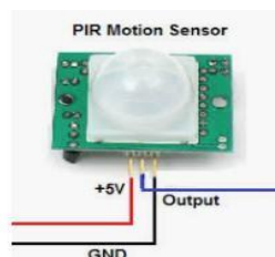
Fig 3 PIR sensor [6]
